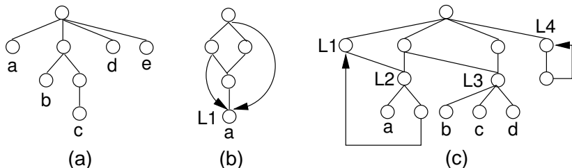
Figure 12.19 Some example multilists.
