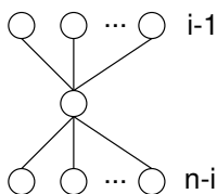
Figure 15.3 The poset that represents the minimum information necessary to determine the i th element in a list. We need to know which element has i - 1 values less and n - i values more, but we do not need to know the relationships among the elements with values less or greater than the i th element.
