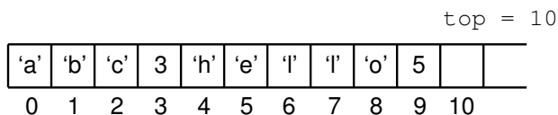
Figure 4.32 An array-based stack storing variable-length strings. Each position stores either one character or the length of the string immediately to the left of it in the stack.
