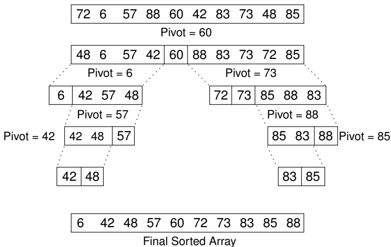
Figure 7.9 An illustration of Quicksort.
