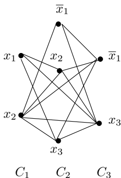
Figure 17.4 The graph generated from boolean expression B = (x_1 + x_2) \cdot (\bar{x}_1 + x_2 + x_3) \cdot (\bar{x}_1 + x_3) . Literals from the first clause are labeled C_1 , and literals from the second clause are labeled C_2 . There is an edge between every two pairs of vertices except when both vertices represent instances of literals from the same clause, or a negation of the same variable. Thus, the vertex labeled C_1 : y_1 does not connect to the vertex labeled C_1 : y_2 (because they are literals in the same clause) or the vertex labeled C_2 : \bar{y}_1 (because they are opposite values for the same variable).
