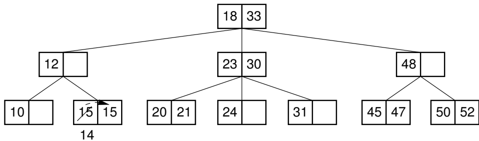
Figure 10.11 Simple insert into the 2-3 tree of Figure 10.9. The value 14 is inserted into the tree at the leaf node containing 15. Because there is room in the node for a second key, it is simply added to the left position with 15 moved to the right position.
