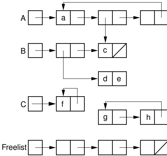
Figure 12.16 Example of LISP list variables, including the system freelist.
