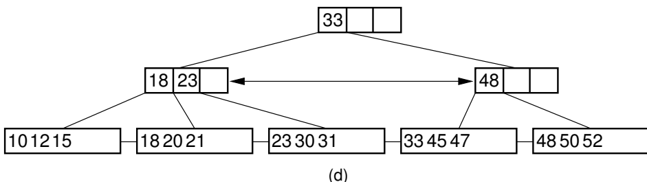
Figure 10.18 Examples of B + -tree insertion. (a) A B + -tree containing five records. (b) The result of inserting a record with key value 50 into the tree of (a). The leaf node splits, causing creation of the first internal node. (c) The B + -tree of (b) after further insertions. (d) The result of inserting a record with key value 30 into the tree of (c). The second leaf node splits, which causes the internal node to split in turn, creating a new root.
